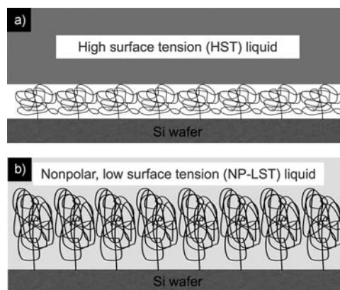
Figure 1. Illustration of two different types of “liquid–liquid interfaces” between the probe liquids and the PDMS brush-film surfaces.
